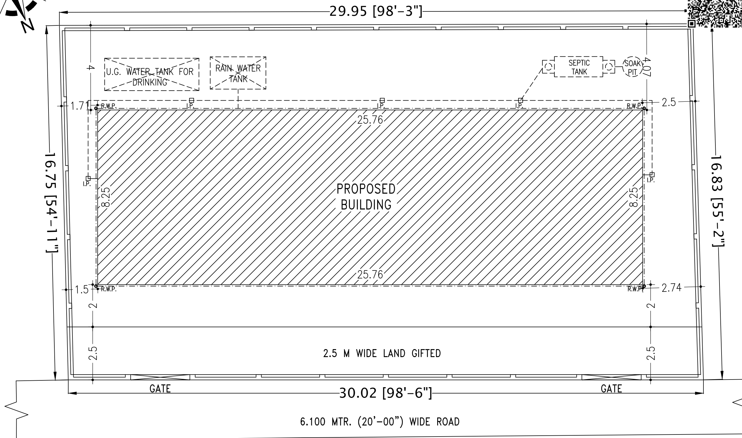
WATER & SEWERAGE PLAN SCALE - 1:200
